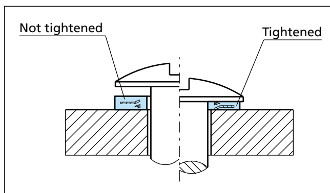
Figure 30 Installation Seloc
