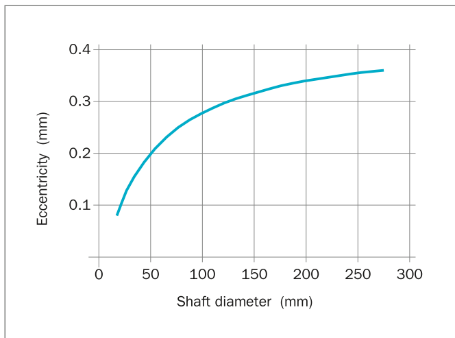
Figure 61: Permissible eccentricity
